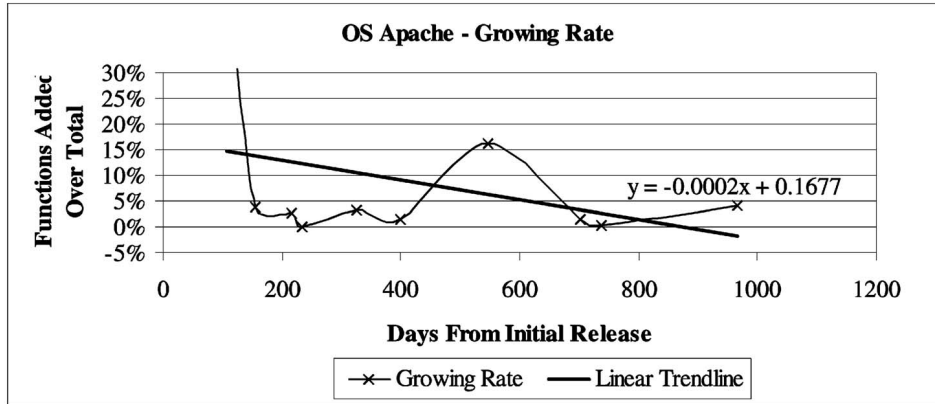
Fig. 2. Growing rate of apache over time.
