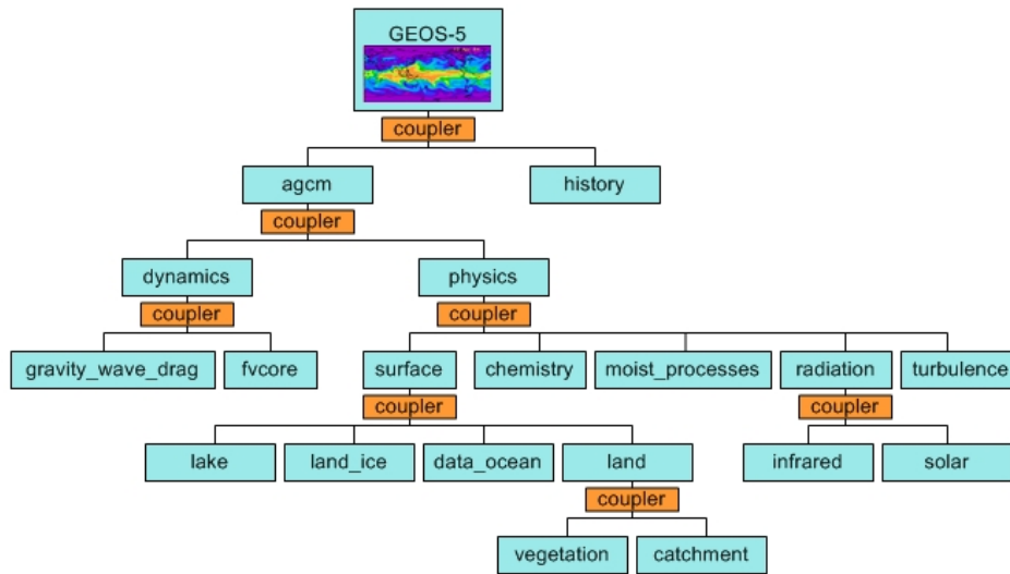
Figure 3: Earth System Modeling Framework (ESMF) component architecture of the Goddard Earth Observing System, version 5 (GEOS-5) atmospheric model ( http://www.esmf.ucar.edu/about_us/ ). See text for detailed discussion.
