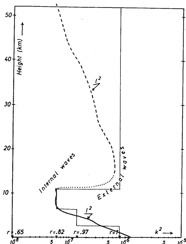
Fig. 5. l^2 as function of height. Solid line is computed from observed winds and temperatures in the Sierra Nevada regions, dashed line from the mean values of wind and temperature, and dotted line is obtained by interpolation. The l^2 -curve separates the regions of internal and external waves. Thin line shows the values of l^2 for a four-layer model.
