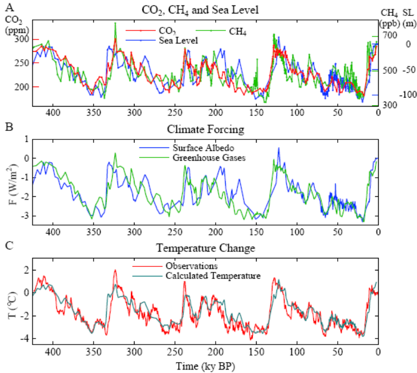
Fig. 1. (A) CO 2 , CH 4 (16) and sea level (17) for past 425 ky. (B) Climate forcings due to changes of GHGs and ice sheet area, the latter inferred from sea level from land level change. (C) Calculated global temperature change based on climate sensitivity of 3/4°C per W/m 2 . Observations are Antarctic temperature change (16) divided by two.
