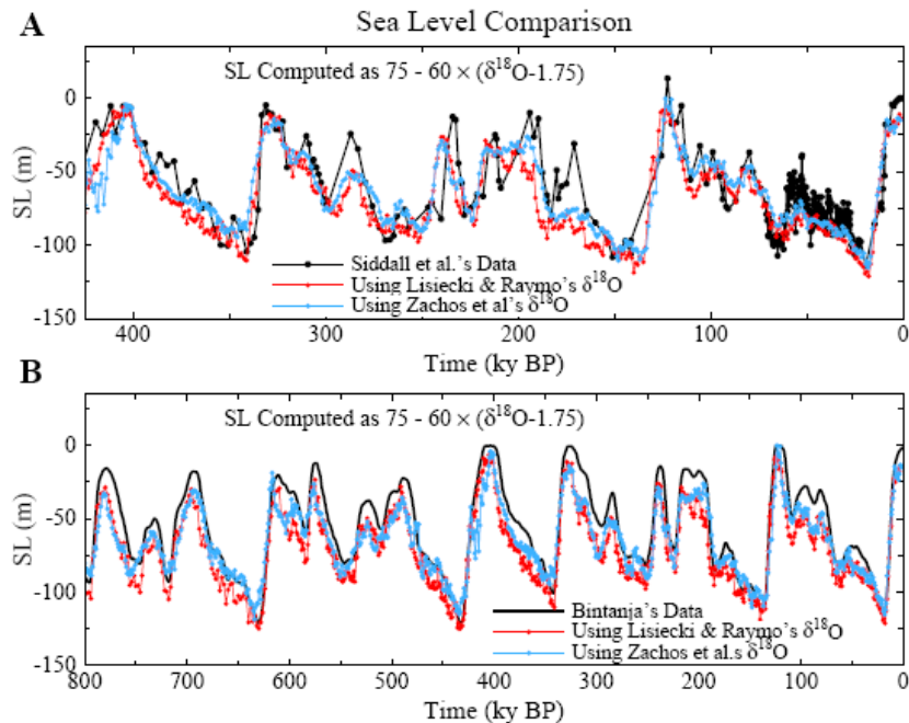
Fig. S8. (A) Comparison of Siddall et al. (17) sea level record with sea level computed from \delta^{18}\text{O} via Eq. S2 using two alternative global benthic stacks (24, S14). (B) Comparison of Bintanja et al. (S15) sea level reconstruction with the same global benthic stacks as in (A).
