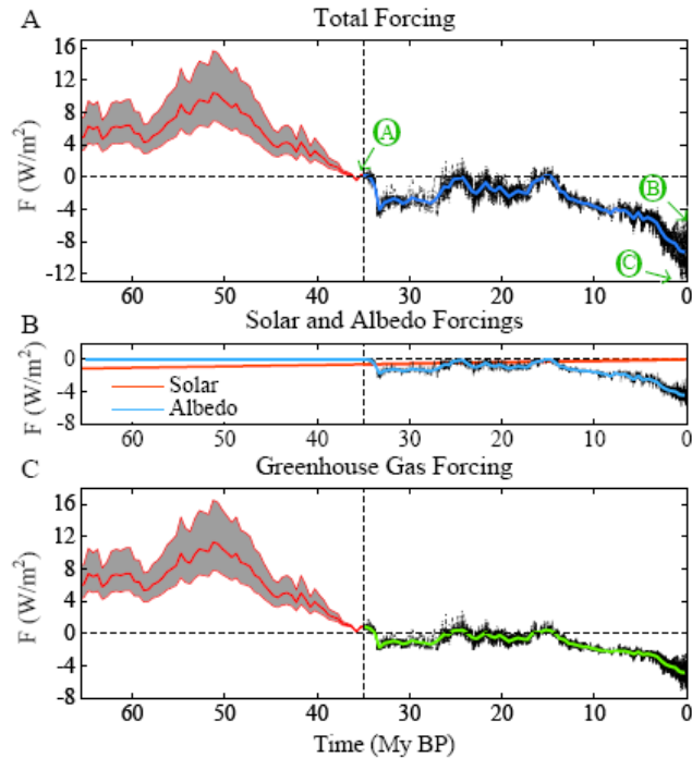
Fig. 4. (A) Total climate forcing, (B) solar and surface albedo forcings, and (C) GHG forcing in the Cenozoic, based on T_{do} history of Fig. 3B and assumed fast-feedback climate sensitivity 3/4^{\circ}\text{C} per \text{W}/\text{m}^2 . Ratio of T_s change and T_{do} change is assumed to be near unity in the minimal ice world between 65 and 35 My, but the gray area allows for 50% uncertainty in the ratio. In the later era with large ice sheets we take T_s/T_{do} = 1.5 , in accord with Pleistocene data.
