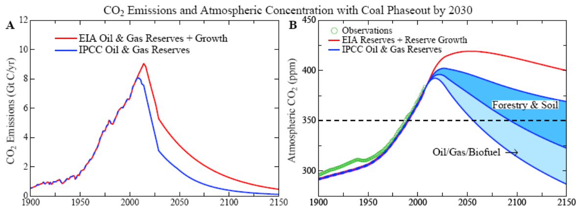
Fig. 6. (A) Fossil fuel CO 2 emissions with coal phase-out by 2030 based on IPCC (2) and EIA (78) estimated fossil fuel reserves. (B) Resulting atmospheric CO 2 based on use of a dynamic-sink pulse response function representation of the Bern carbon cycle model (76, 77).
