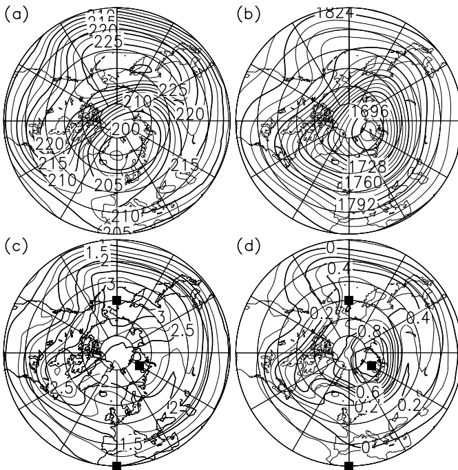
Figure 9. Polar stereographic plots, showing monthly mean fields at 70 hPa in January 2003, north of 30°N: (a) temperature, with contour interval 2.5 K, (b) geopotential height, with interval 8 gpdm, (c) ozone from the SBUV + MIPAS assimilation, with interval 0.25 ppmv, and (d) ozone difference (SBUV + MIPAS minus the SBUV assimilation), with interval 0.1 ppmv. The points marked on (c) and (d) are 75°N 60°E, 60°N 180°E and 30°N 0°E.
